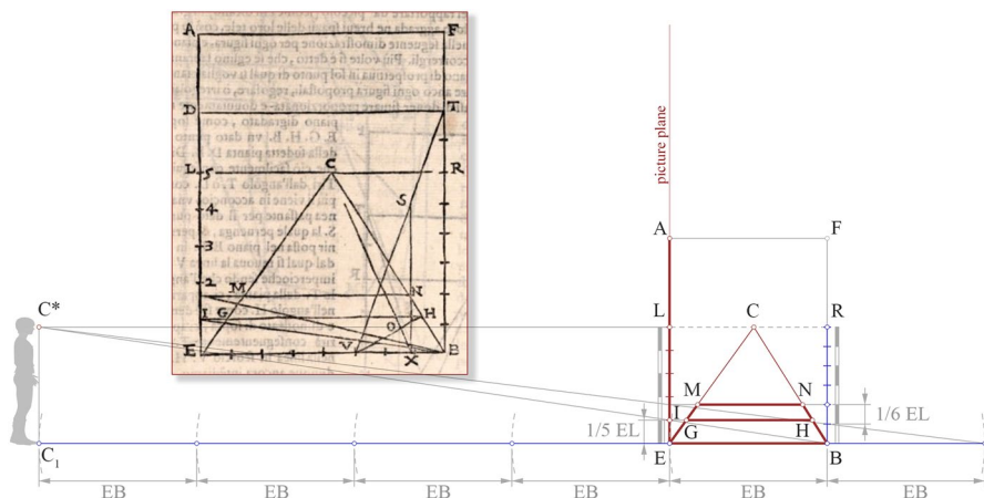
Fig. 5 Pietro Accolti, Come deva il Pittore, quando non può avere il punto della lontananza sudetta, conseguire ad ogni modo gli scorci de' piani, & d'ogni altra figura (What the painter must do, when he cannot have the aforementioned distance point, to achieve in any case the foreshortening of the planes and any other figure). The original figure in page 26, which illustrates the solution of problem in Chapter XIX, is set opposite a scheme which explains the logic of the procedure itself. Image: Accolti (1625: 26)
